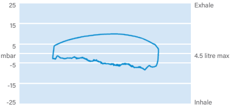
Breathing effort at 50 msw and 50 bar: 0.91 J/l.
